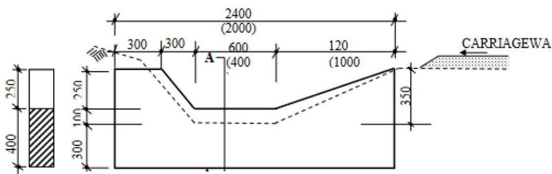
A - A A SECTION OF MASOY SCOUR
