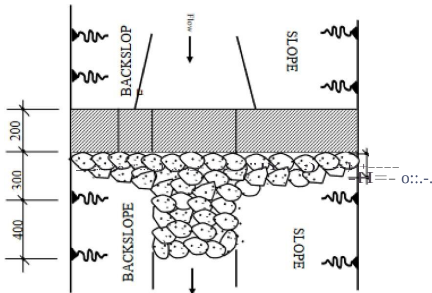
PLAN OF DRAIN WITH EROSION CHECKS QUANTITIES TABLE
