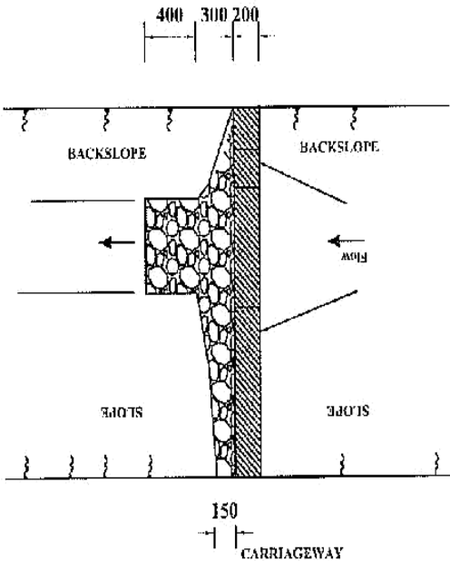
PLAN OF BRAIN WITH SCOUR CHECK
