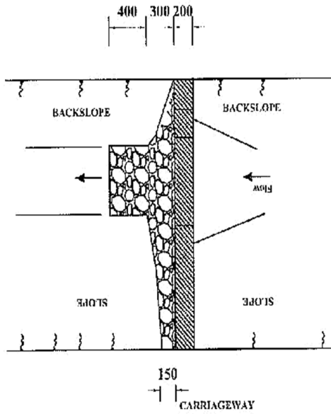
PLAN OF BRIN WITH SCOUR CHECK
