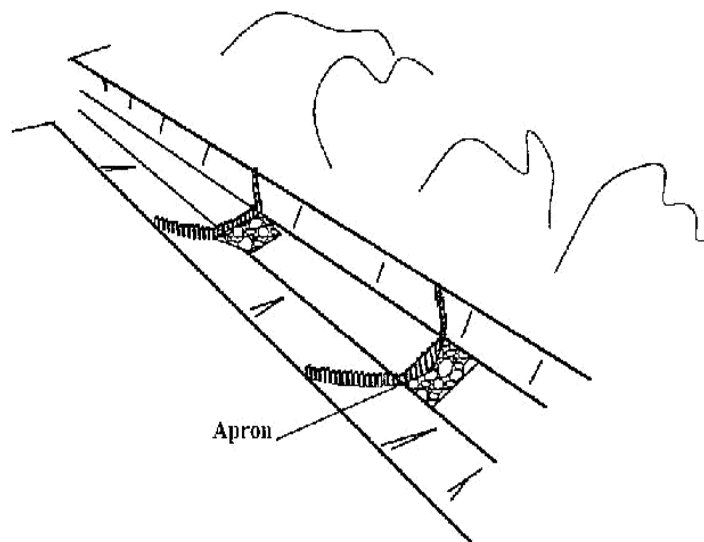
Scour checks made of wooden stakes
