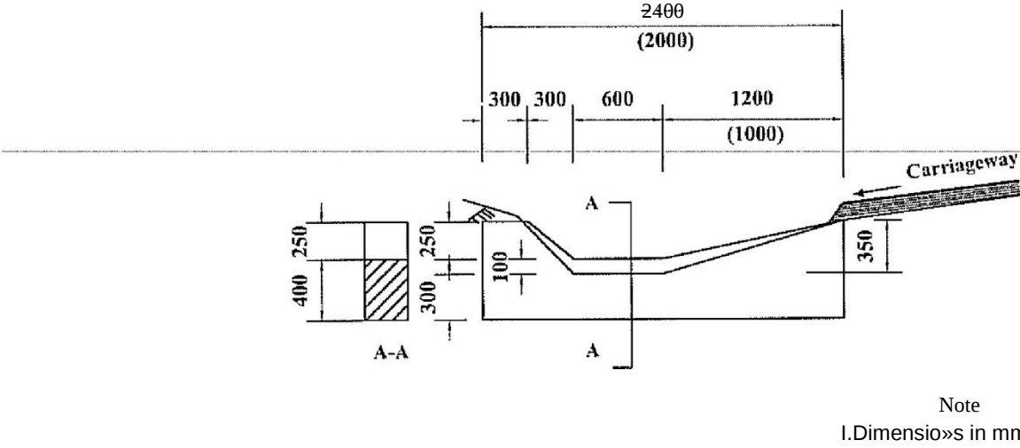
FIGURE C9a-MASONRY SCOUR CHECKS
