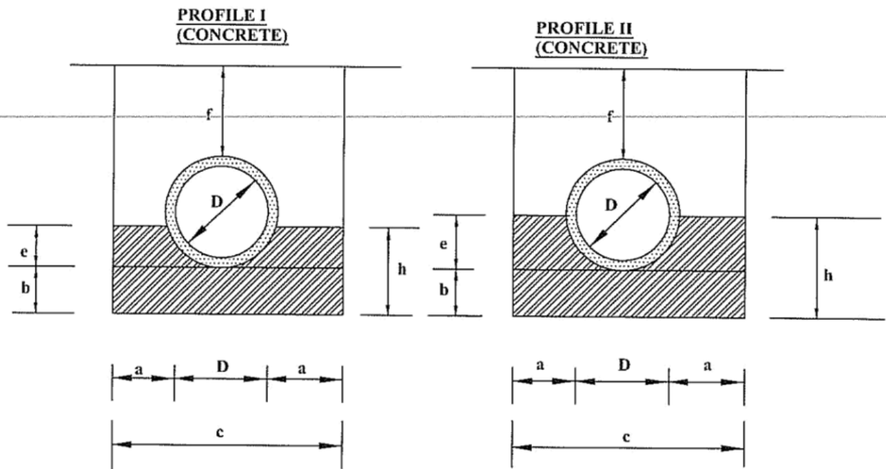
FIGURE C16-BEDDING AND HAUNCH PROFILE TYPES I &amp; II
