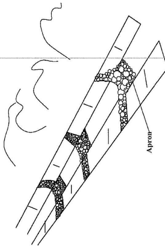
Scour checks made of stones
