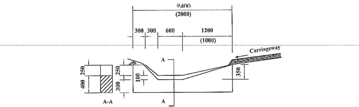
FIGURE C9a-MASONRY SCOUR CHECKS
