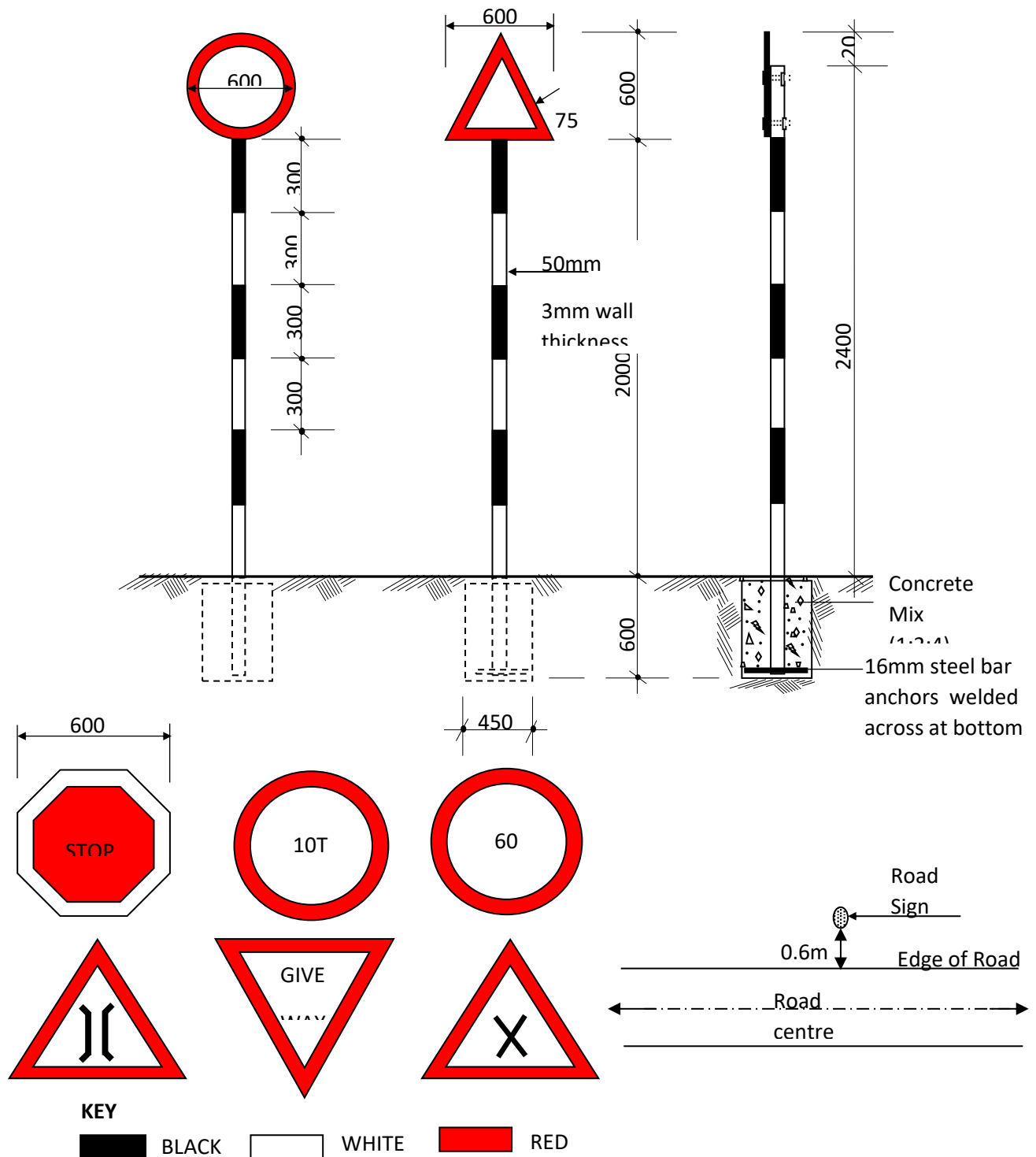
FIGURE C.6 - TRAFFIC SIGNS
