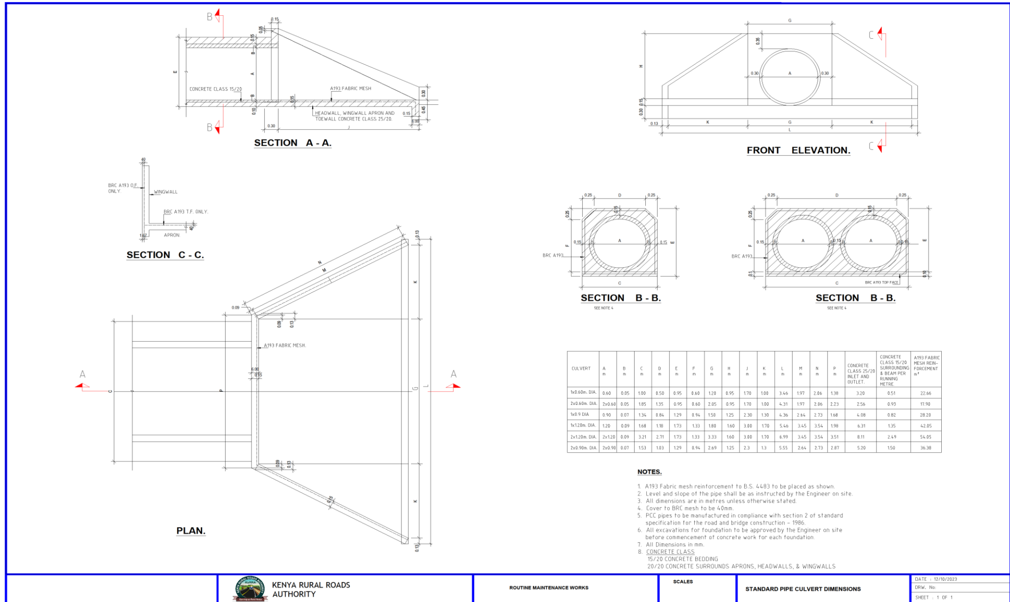
FIGURE C.5 – STANDARD PIPE CULVERT DIMENSIONS
