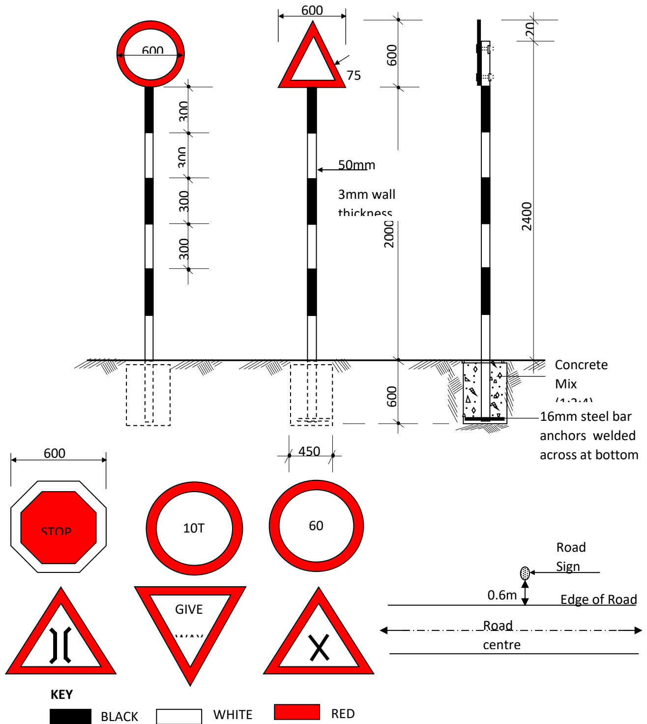
FIGURE C.6 - TRAFFIC SIGNS
