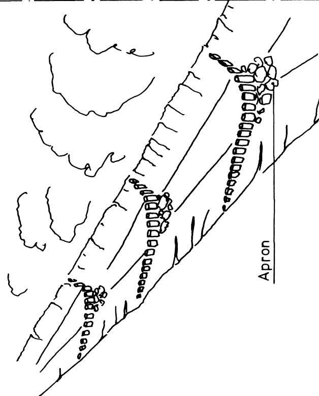
Scour checks made of wooden stakes:
