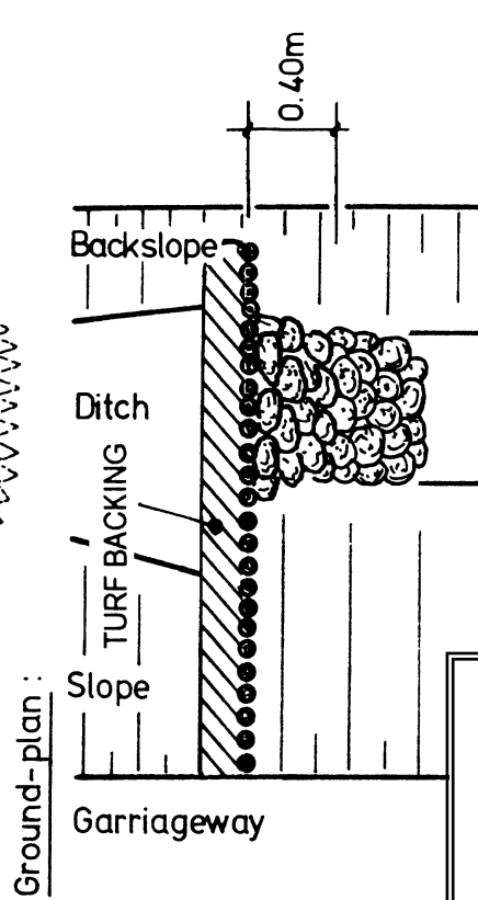
FIGURE C.4 - DIMENSIONS OF SCOUR CHECKS FOR STANDARD DRAIN
