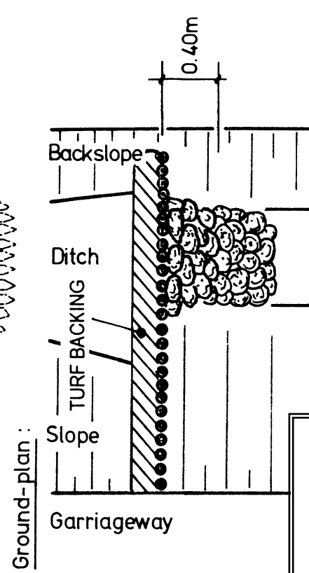
FIGURE C.4 - DIMENSIONS OF SCOUR CHECKS FOR STANDARD DRAIN
