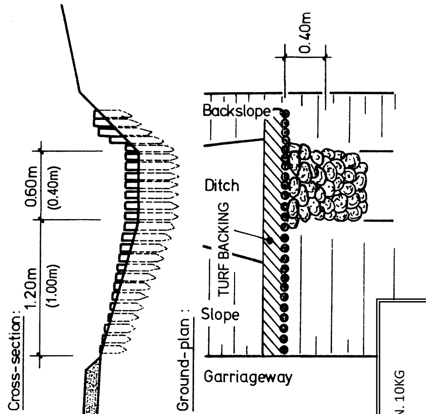
FIGURE C.4 - DIMENSIONS OF SCOUR CHECKS FOR STANDARD DRAIN
