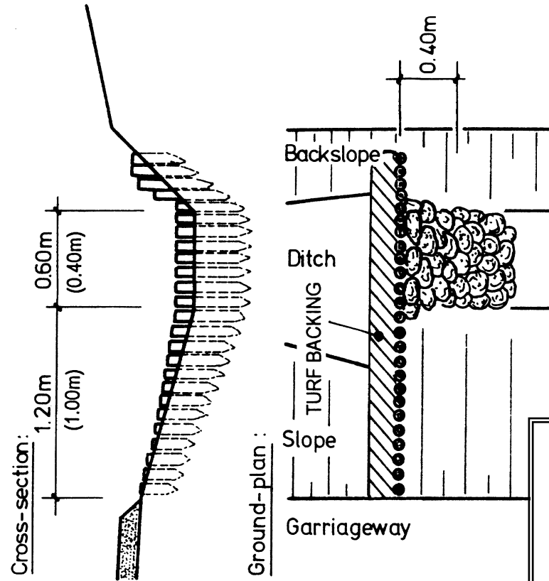
FIGURE C.4 - DIMENSIONS OF SCOUR CHECKS FOR STANDARD DRAIN
