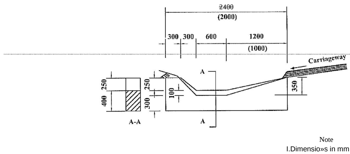
FIGURE C9a-MASONRY SCOUR CHECKS
