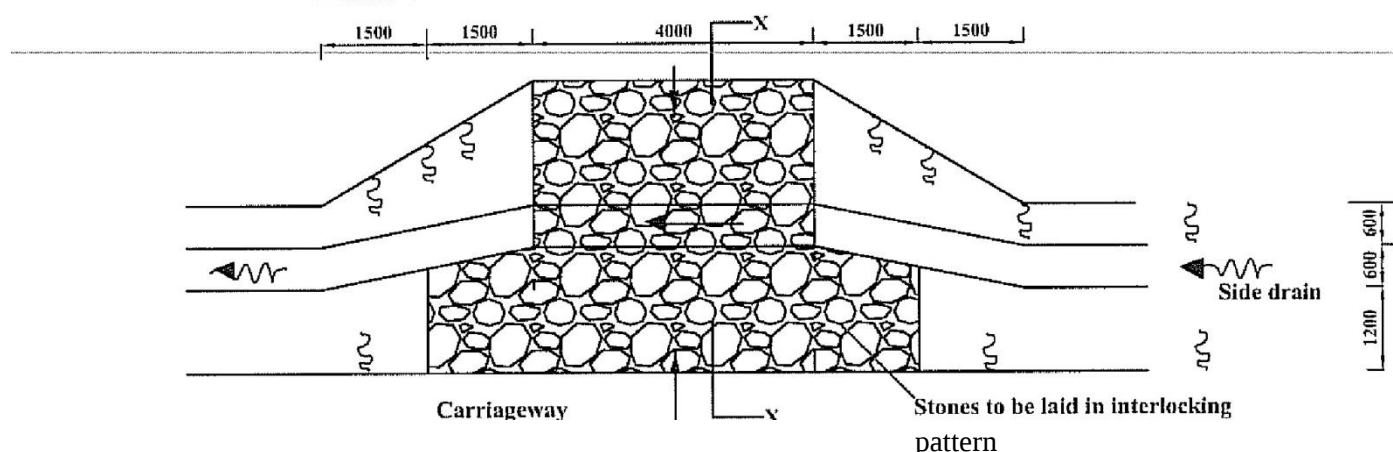
FIGURE C18-ACCESS DRIFT PLAN
