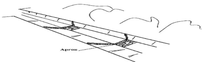
Scour checks made of wooden stakes
