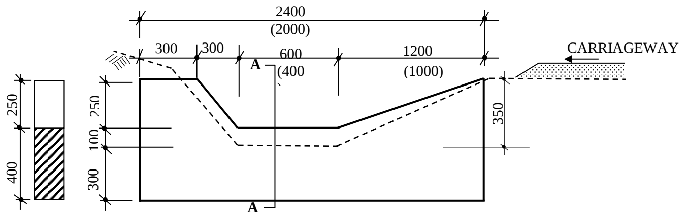
A SECTION OF MASONRY SCOUR CHECKS
