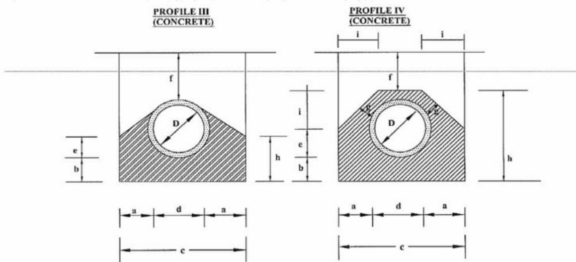
FIGURE C17-BEDDING AND SURROUND PROFILE TYPES III &amp; IV
