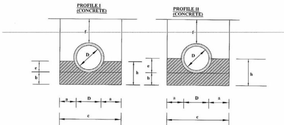
FIGURE C16-BEDDING AND HAUNCH PROFILE TYPES I &amp; II
