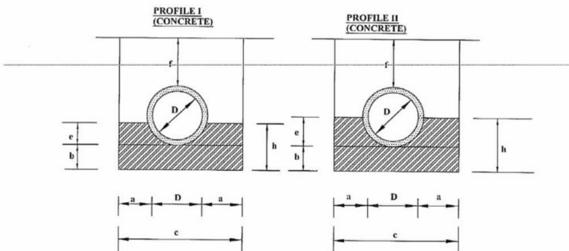
FIGURE C16-BEDDING AND HAUNCH PROFILE TYPES I &amp; II
