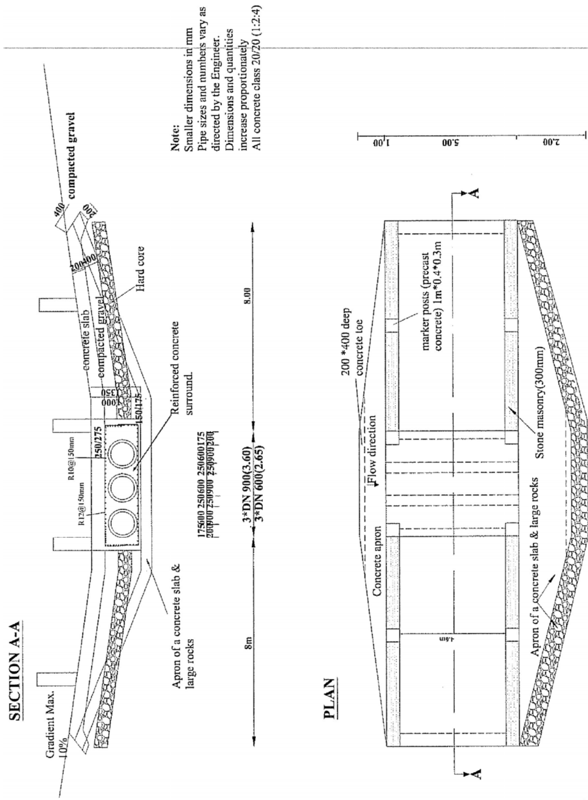
FIGURE C20-VENTED DRIFT
