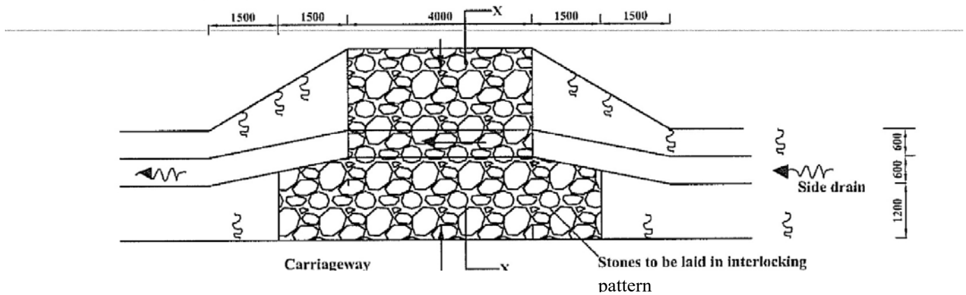
FIGURE C18-ACCESS DRIFT PLAN
