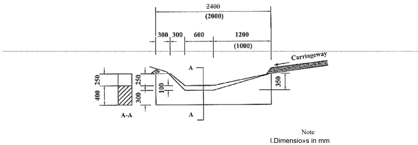
FIGURE C9a-MASONRY SCOUR CHECKS
