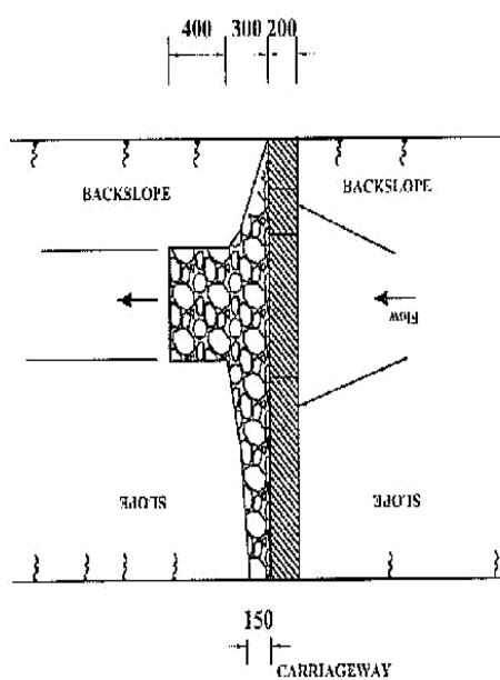
PLAN OF DRAIN WITH SCOUR CHECK
