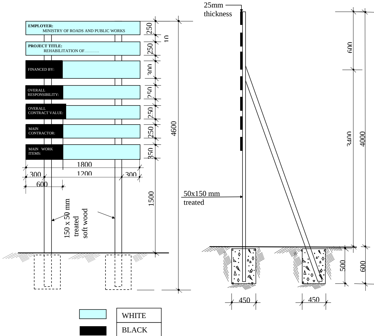
FIGURE C.17 - PUBLICITY SIGNBOARD
