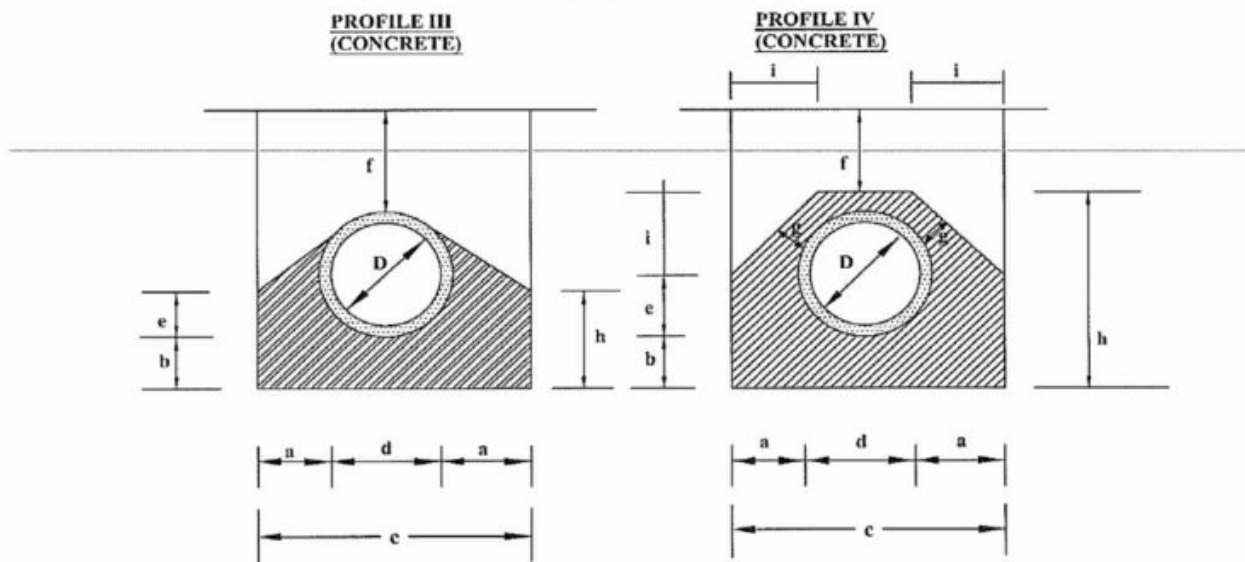
FIGURE C17-BEDDING AND SURROUND PROFILE TYPES III &amp; IV
