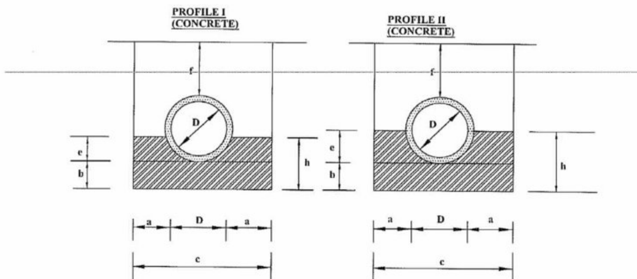
FIGURE C16-BEDDING AND HAUNCH PROFILE TYPES I &amp; II
