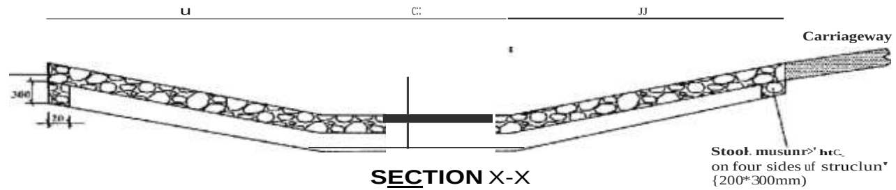
150mm Groufed Stone Pitching (Cement mortar 1:4)
