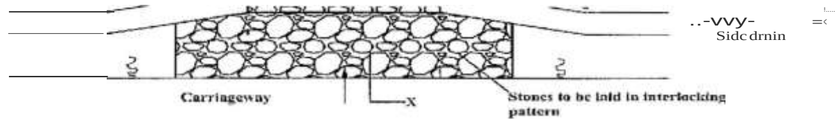
150mm Groufed Stone Pitching (Cement mortar 1:4)
