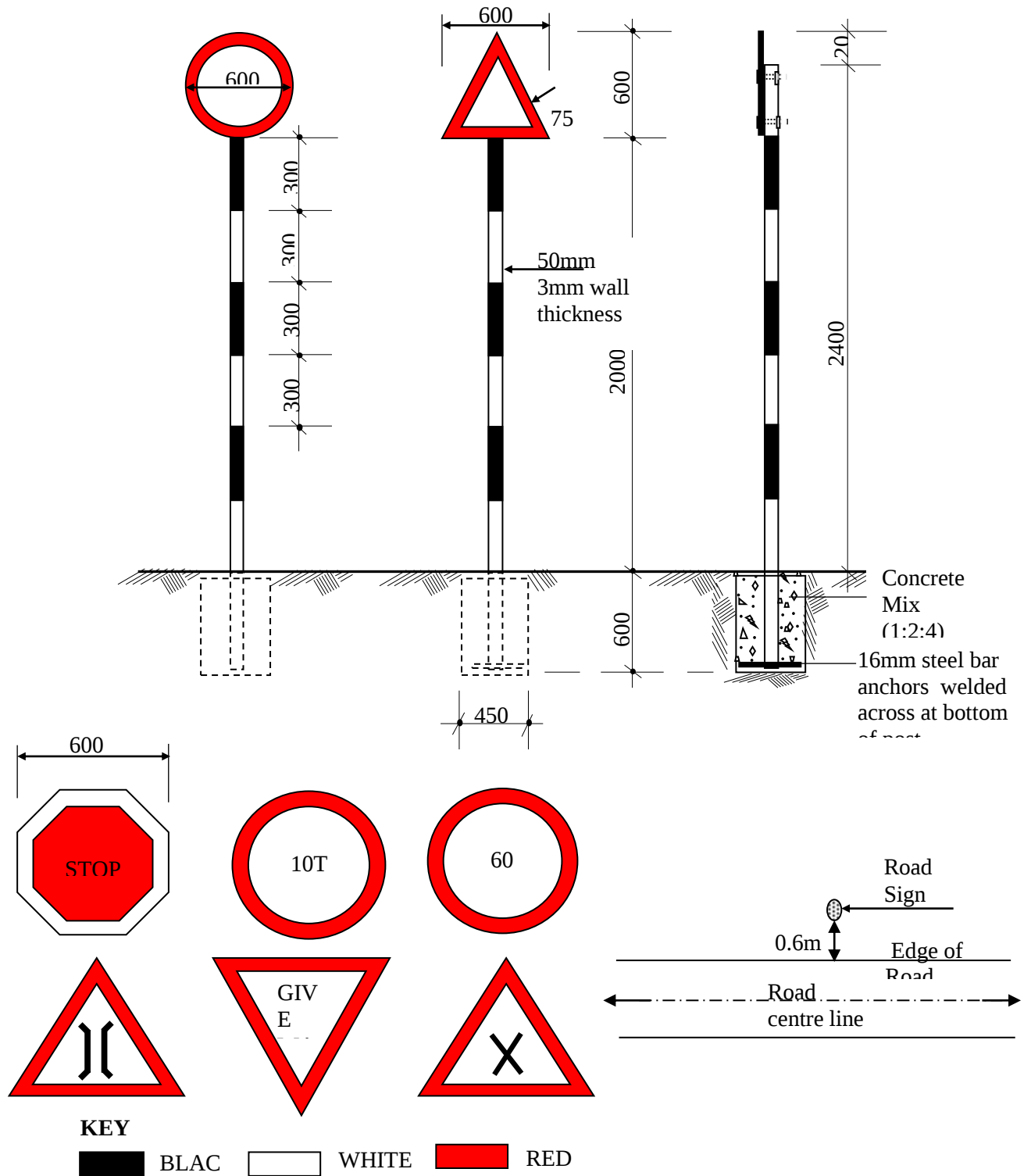
FIGURE C.16 - TRAFFIC SIGNS
