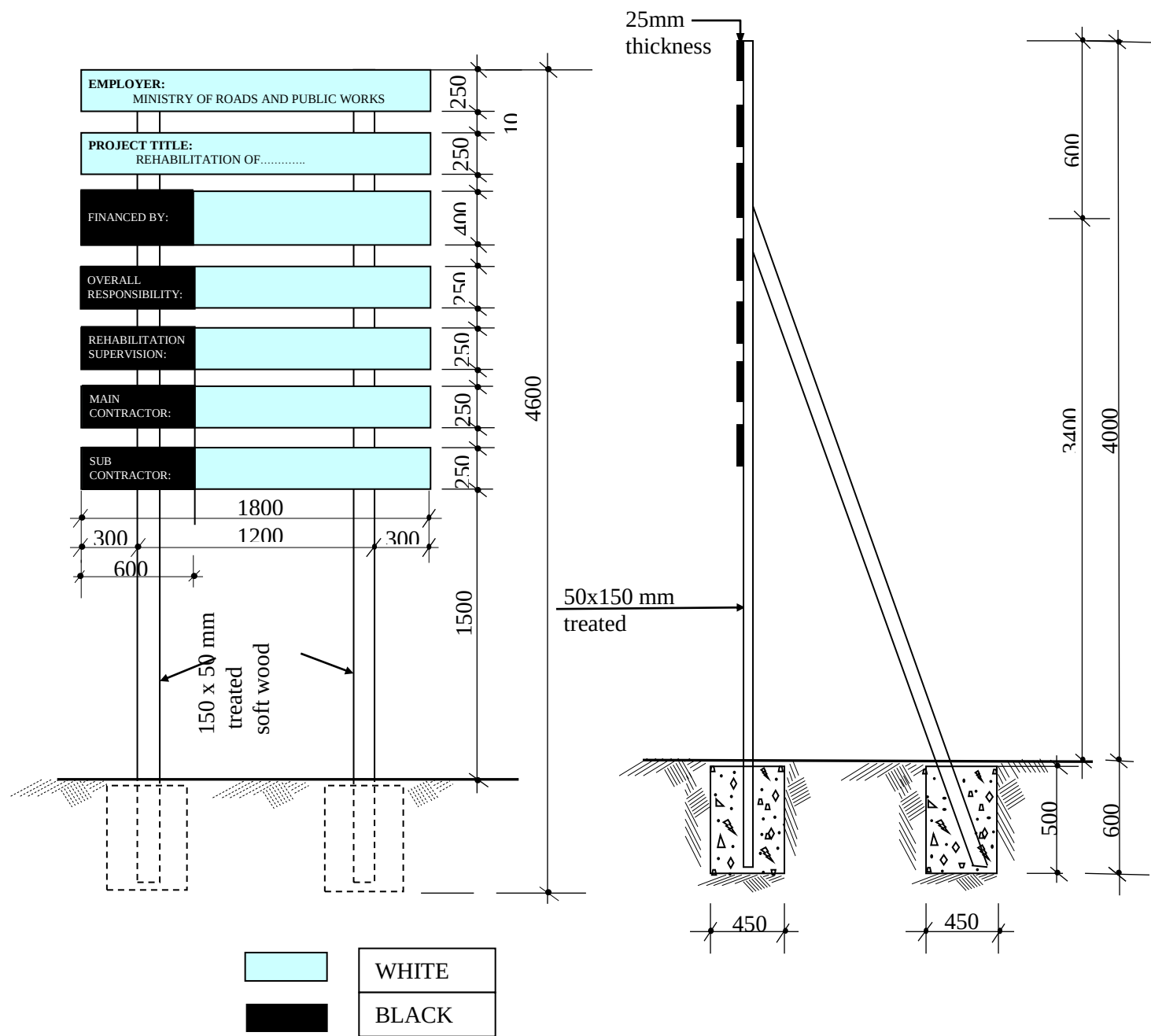
FIGURE C.17 - PUBLICITY SIGN BOARD
