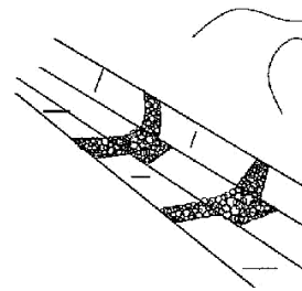
Scour checks made of stones
