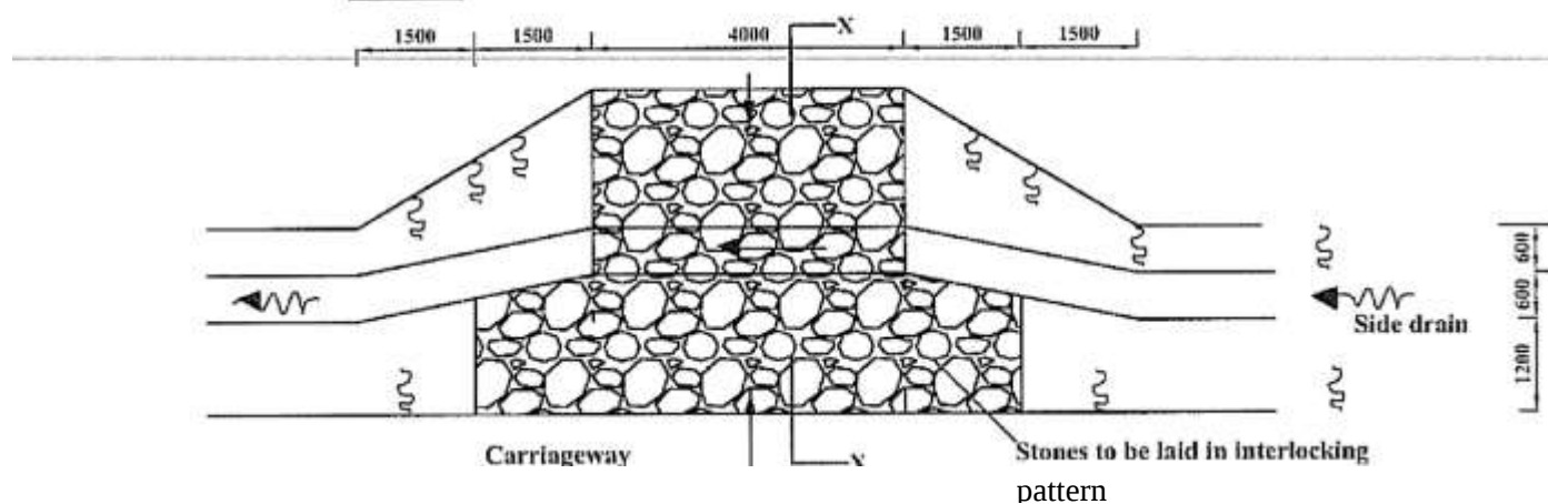
FIGURE C18-ACCESS DRIFT PLAN
