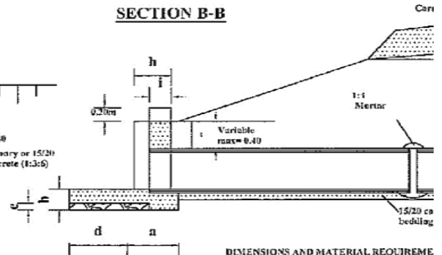
DIMENSIONS AND MATERIAL REQUIREMENT
