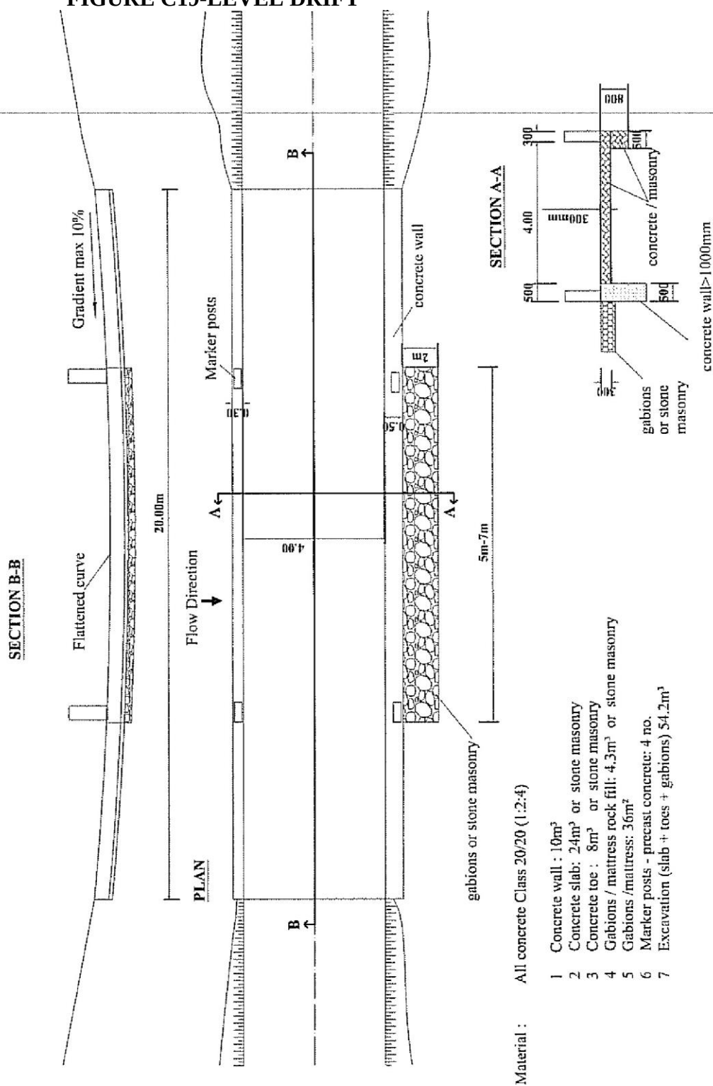
FIGURE C19-LEVEL DRIFT
