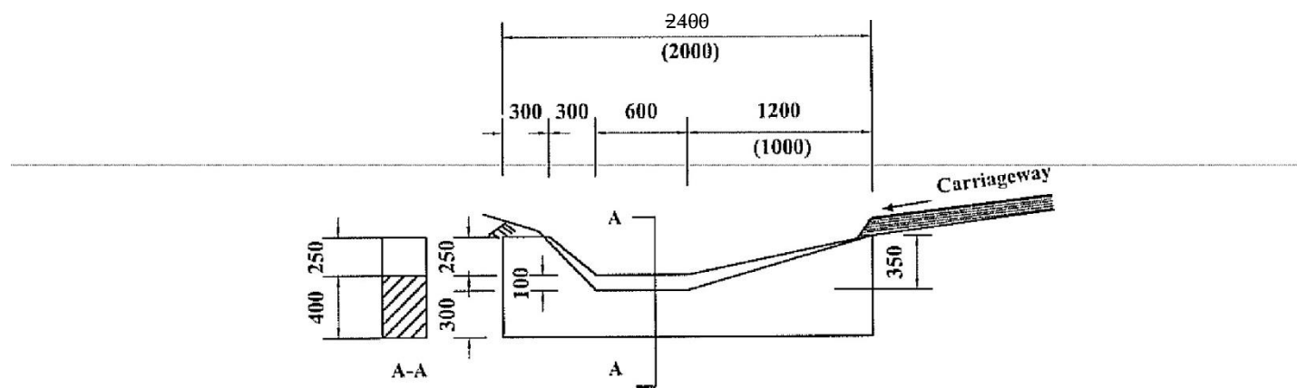
FIGURE C9a-MASONRY SCOUR CHECKS
