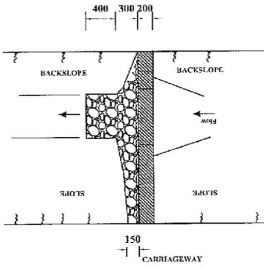
PLAN OF DRAIN WITH SCOUR CHECK
