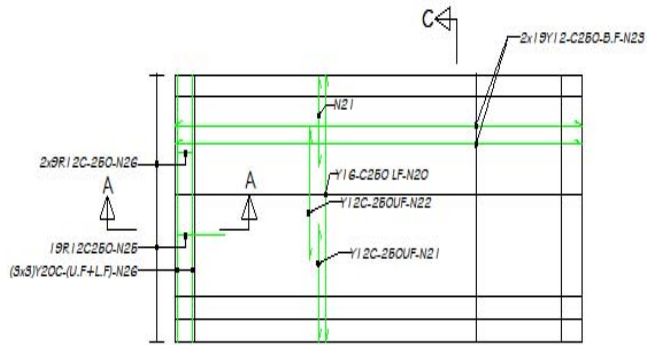
TOP SLAB REINFORCEMENT
