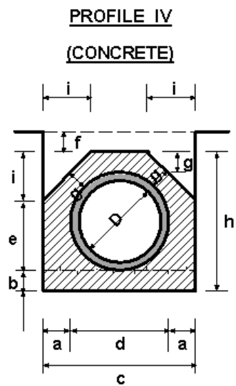
FIGURE C.14 - BEDDING AND HAUNCH PROFILES TYPES III & IV
