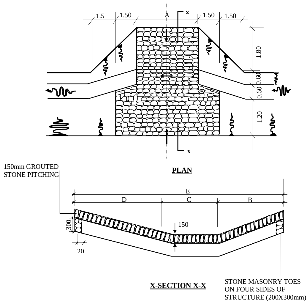
FIGURE C.15 ACCESS DRIFT
