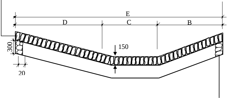
X-SECTION X-X
