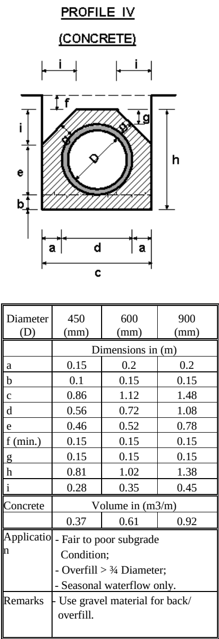
FIGURE C.14 - BEDDING AND HAUNCH PROFILES TYPES III & IV
