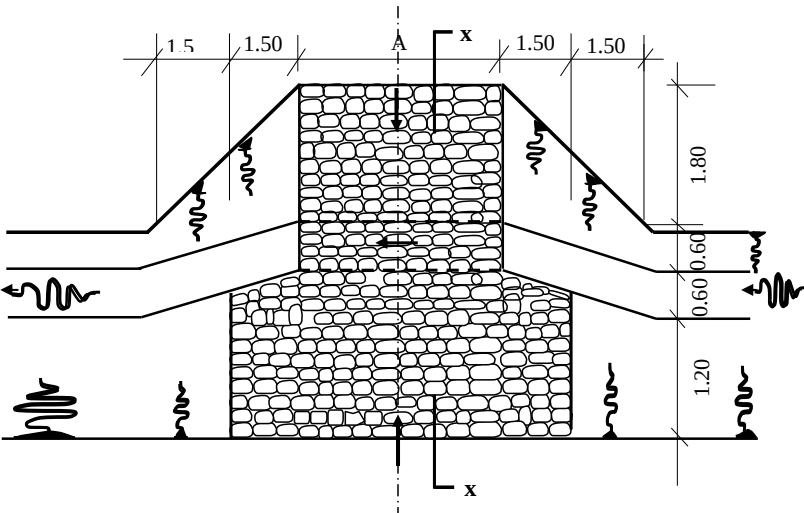
FIGURE C.15 ACCESS DRIFT
