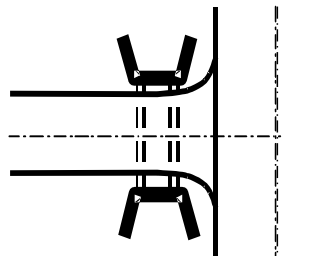
TYPE 4 (ENTRY AND EXIT ON ACCESS)
