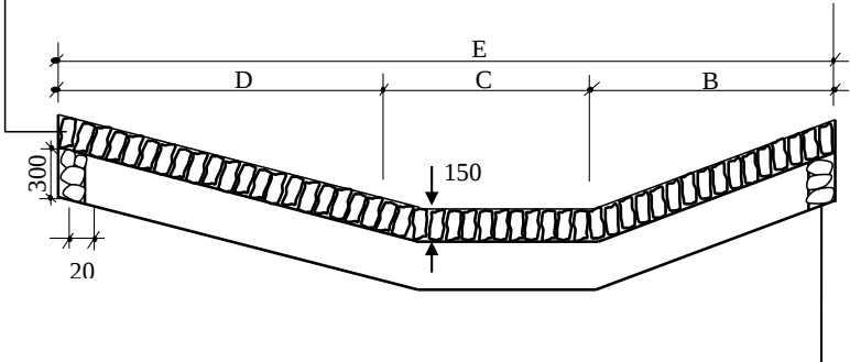
X-SECTION X-X
