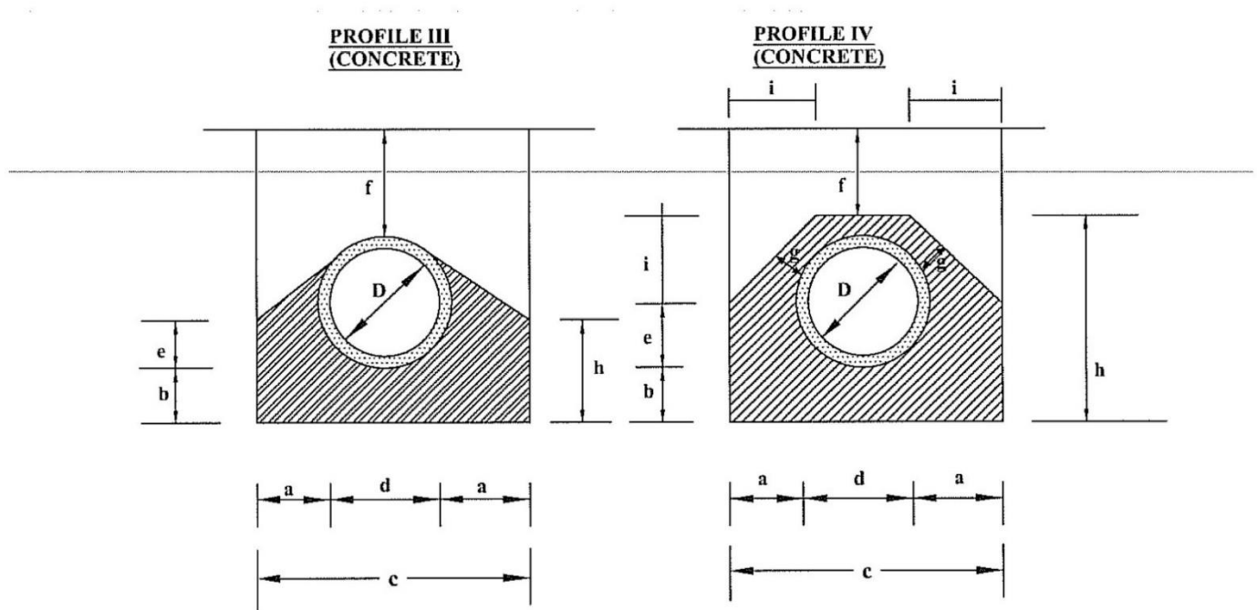
FIGURE C17-BEDDING AND SURROUND PROFILE TYPES III & IV
