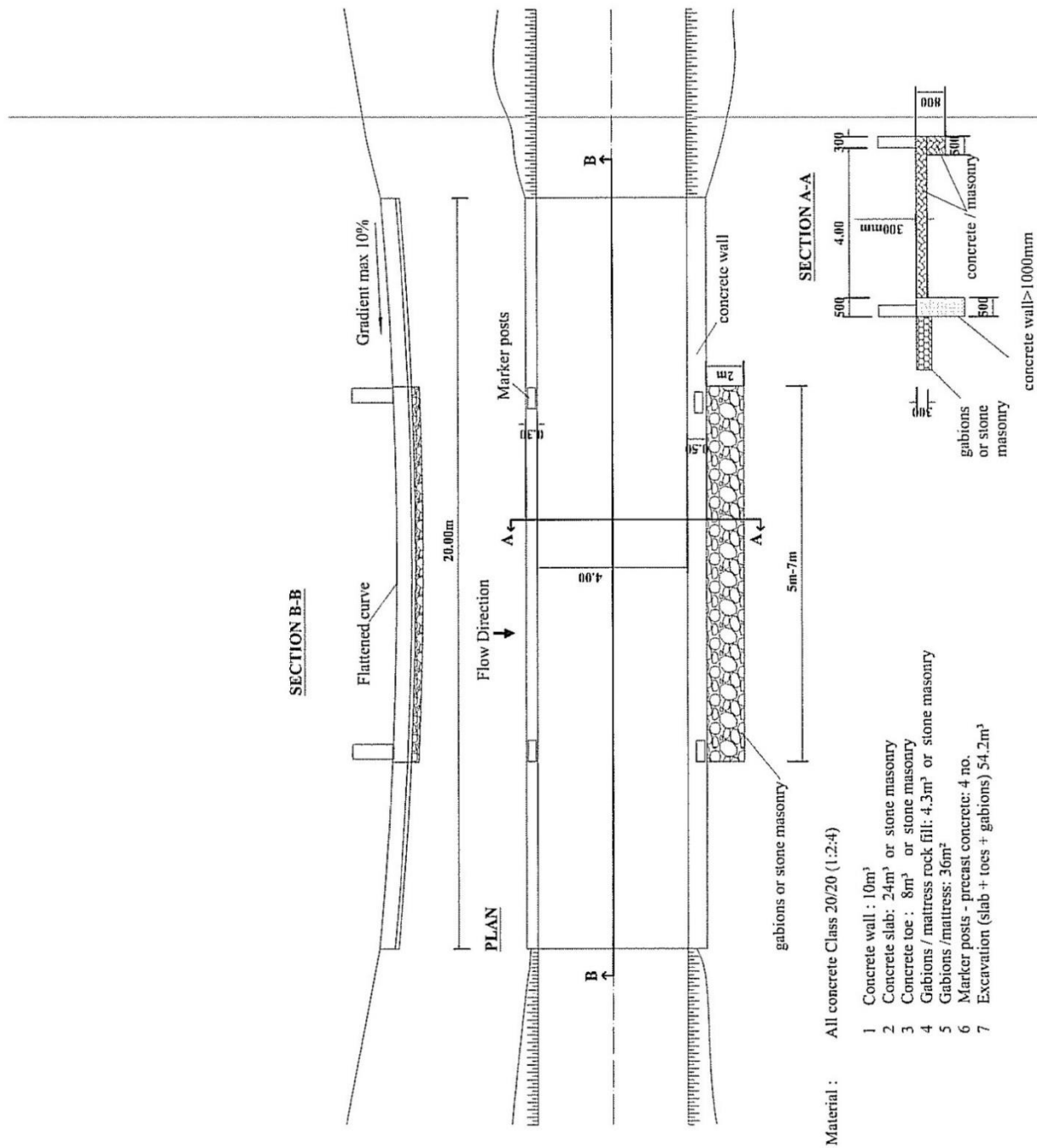
FIGURE C19-LEVEL DRIFT
