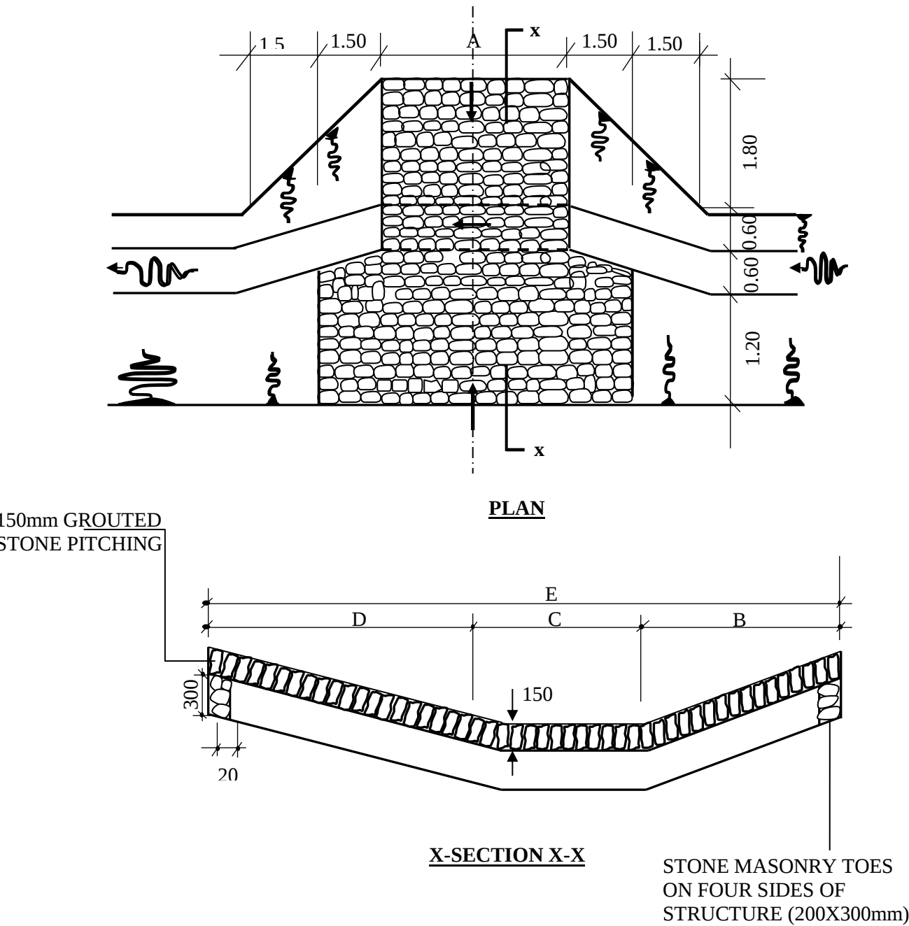
FIGURE C.15 ACCESS DRIFT
