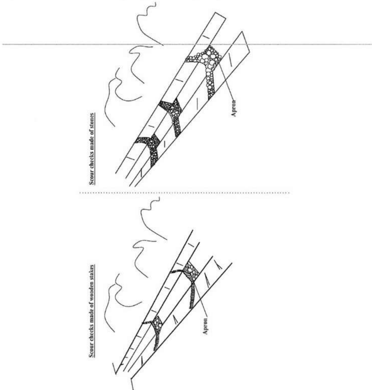
FIGURE C.7 SCOUR CHECKS
