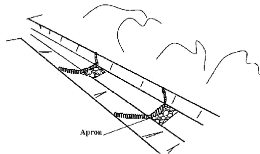
Scour checks made of wooden shingles
