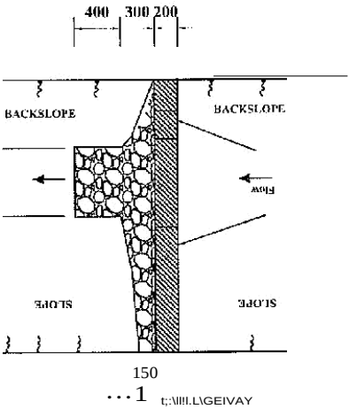
SECTION OF MASONRY SCOUR CHECK
