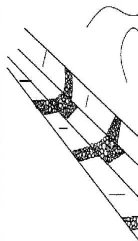
Scour checks made of stones
