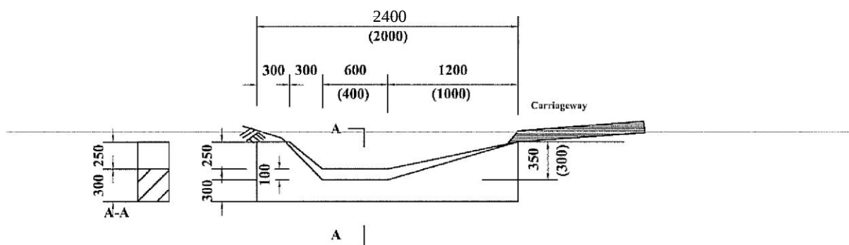
SECTION OF CONCRETE SCOUR CHECK
