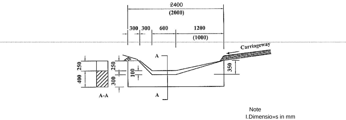
SECTION OF MASONRY SCOUR CHECK
