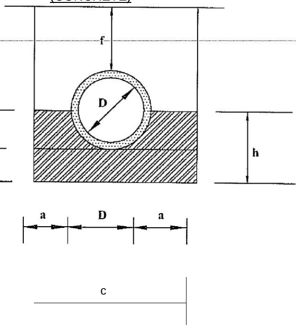
PROFILE 11 (CONCRETE)
