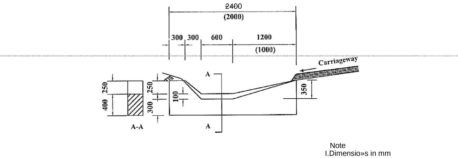
SECTION OF MASONRY SCOUR CHECK
