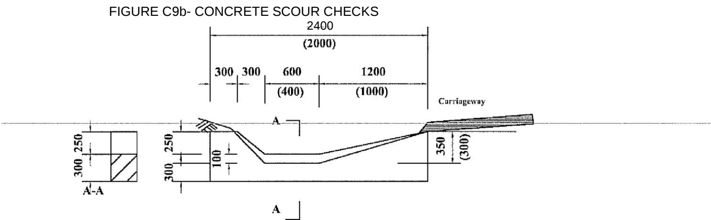
SECTION OF CONCRETE SCOUR CHECK
