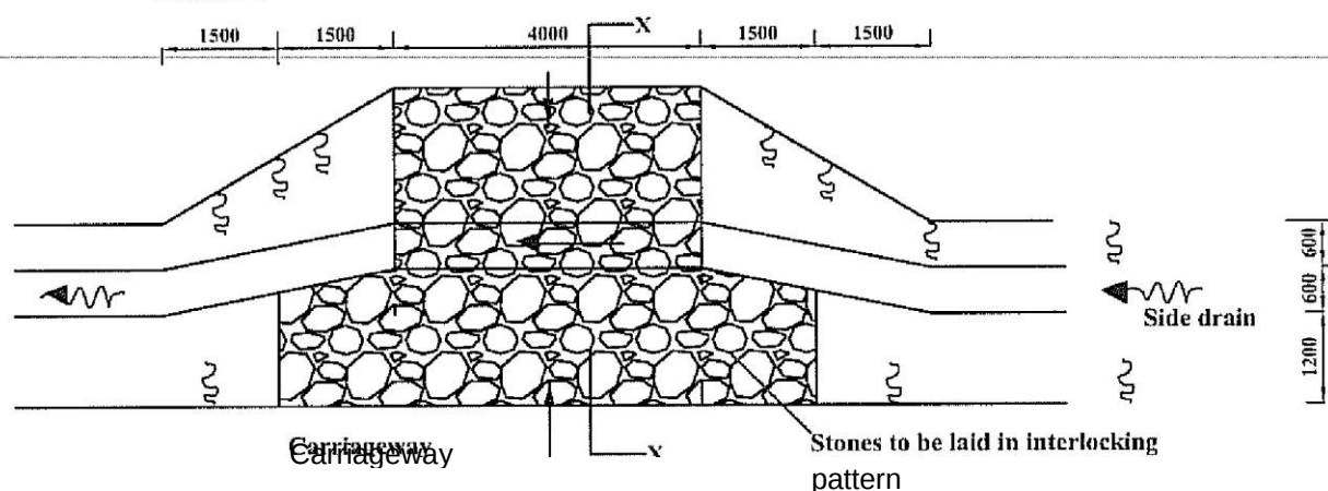
FIGURE C18-ACCESS DRIFT
