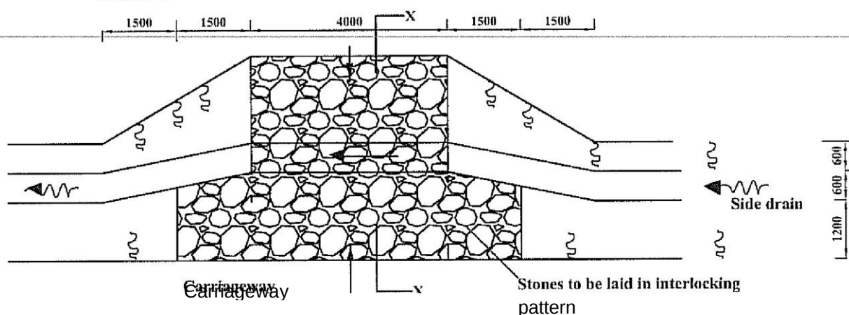
FIGURE C18-ACCESS DRIFT
