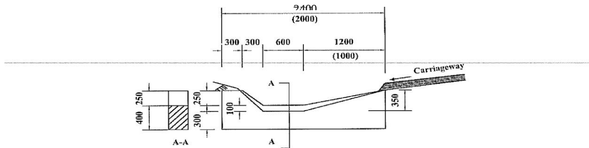
Figure C9a-Masonry Scour Checks
