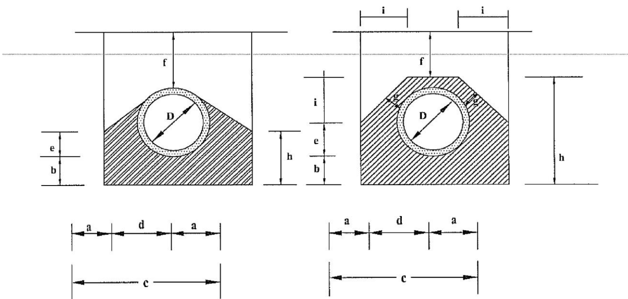
FIGURE C17-BEDDING AND SORROUND PROFILE TYPES III &amp; IV
