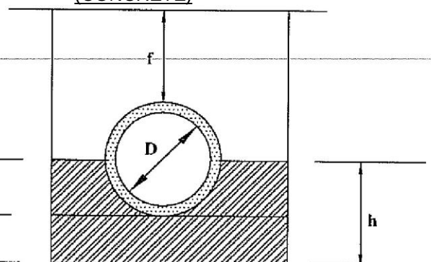
PROFILE 11 (CONCRETE)
